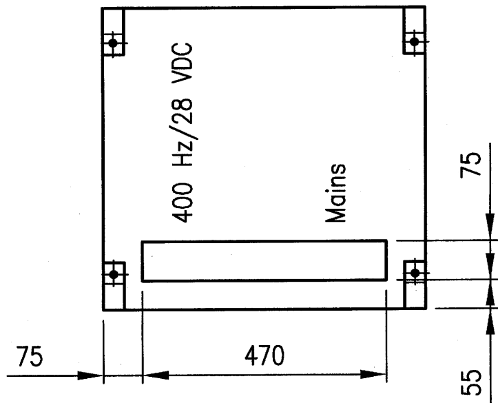
Foundation plan
